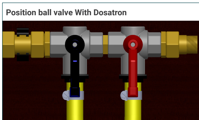
Water control unit \frac{3}{4} " (N°30.00.51001)
