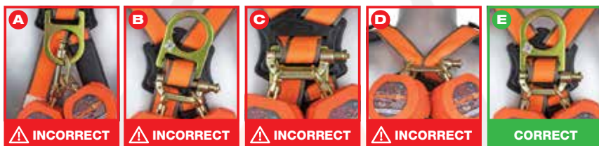
! Figure 5B: Incorrect Twin-leg SRL-P Attachment !
